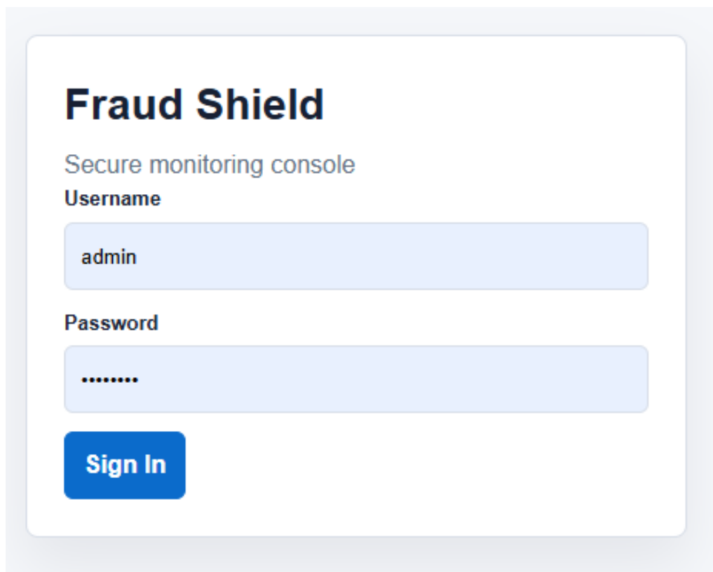
Figure 5.3: Login Page
